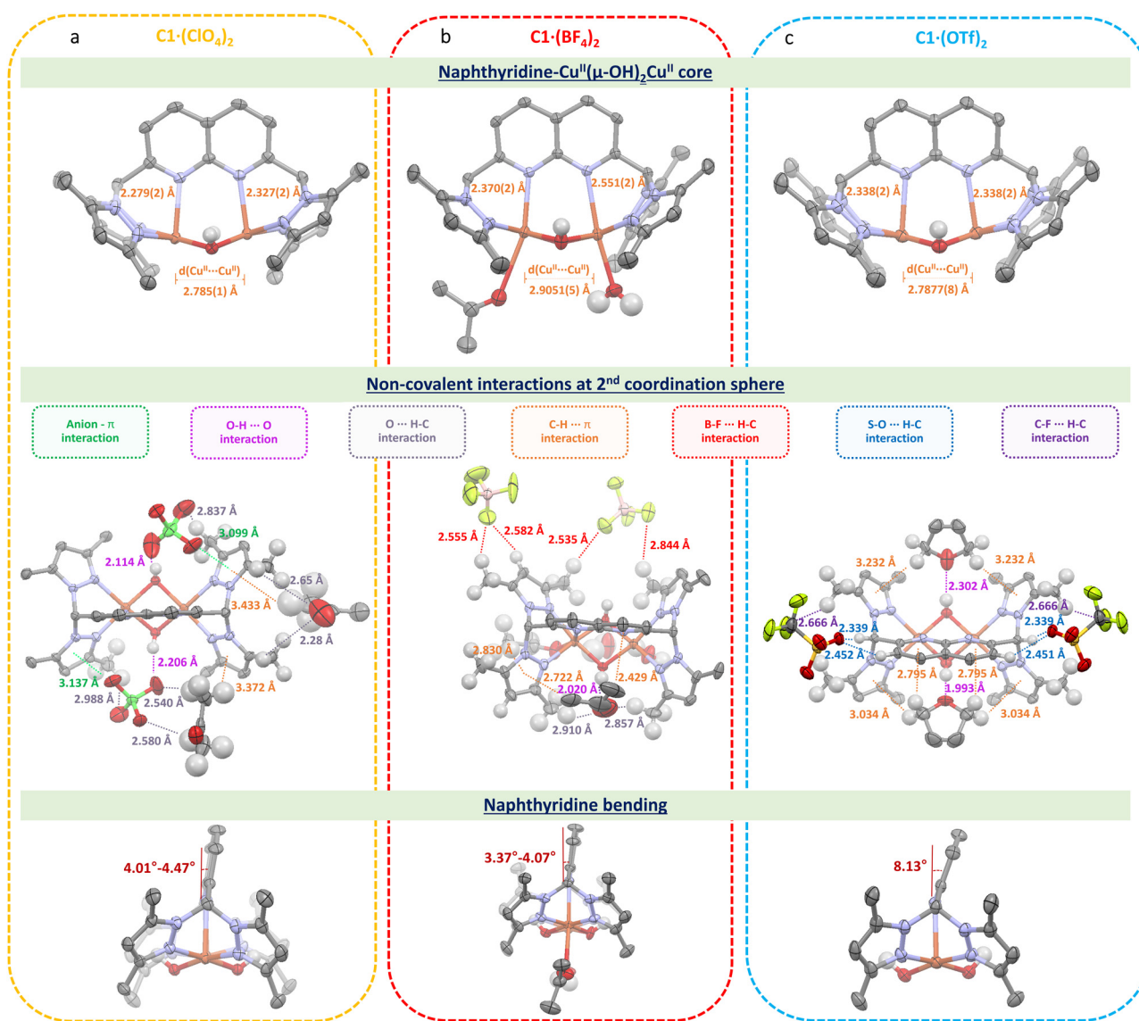
Fig. 1 Displacement ellipsoid plots of (a) C1·(ClO 4 ) 2 , (b) C1·(BF 4 ) 2 and (c) C1·(OTf) 2 complexes at the 50% probability level. Cu–N naph and Cu···Cu distances (top), non-covalent interactions (middle) and naphthyridine bending angles (bottom). Solvent molecules, free anions and hydrogen atoms (except for the O–H bridges or when discussed) are omitted for clarity.
