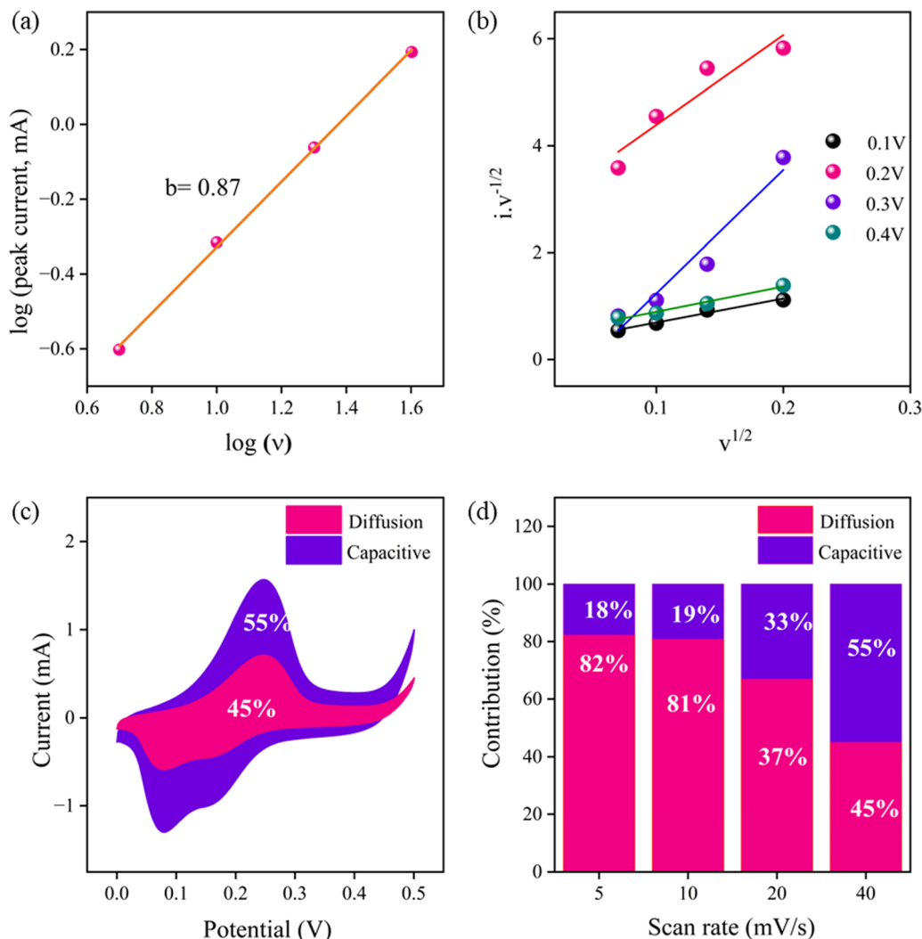
Fig. 4 (a) \log(i_p) vs. \log(v) profile for finding the b -value. (b) i_p v^{-1/2} vs. v^{1/2} profile. (c) Percentage contribution of surface capacitance and diffusion-controlled capacitance for C-ZIF-800 in 1 M KOH electrolyte at 40 \text{ mV s}^{-1} . (d) Bar diagram representing percentage contributions at various scan rates.
