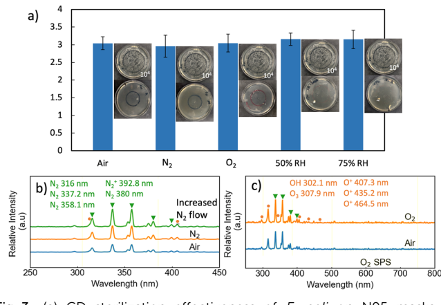
Fig. 3 (a) CD sterilization effectiveness of E. coli on N95 masks at different atmospheres; (b) spectrum generated by CD under N 2 flow; (c) spectrum generated by CD under O 2 flow.
