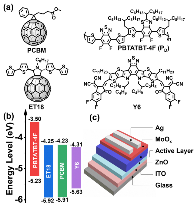
Fig. 1 Chemical structures (a) and HOMO/LUMO energy levels (b) of PBTATBT-4F (hereafter P D ), Y6, ET18, and PCBM. Note, all HOMO energy levels were measured by UPS and the LUMO energy levels calculated by using the optical gap using the equation E_{\text{LUMO}} = E_{\text{HOMO}} + E_{\text{optg}} . (c) Device architecture used in this study.
