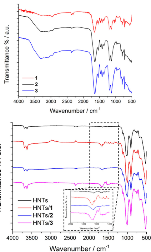
Fig. 4 FT-IR spectra of (a) PNA tetramers 1 , 2 and 3 ; (b) HNTs, HNTs/ 1 , HNTs/ 2 and HNTs/ 3 nanomaterials.
