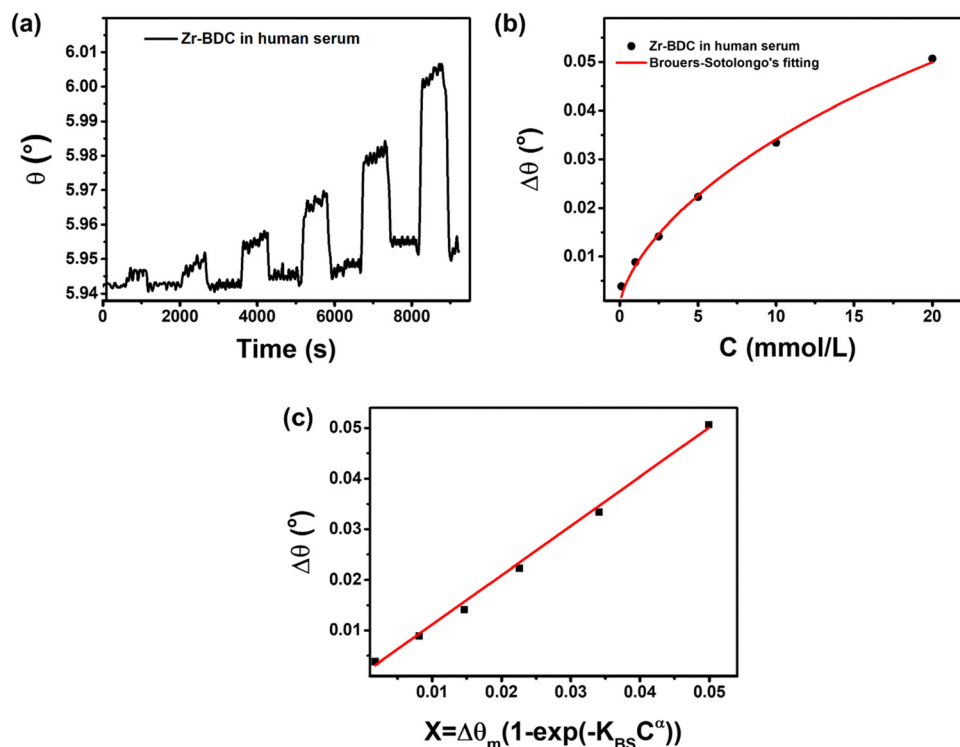
Fig. 8 (a) SPR dynamic response, (b) the Brouers–Sotolongo isotherm adsorption model fitting, and (c) the calibration curve of the hierarchical plate-like Zr-BDC to 0.1 – 20 \text{ mmol L}^{-1} glucose in a human serum/PBS solution.
