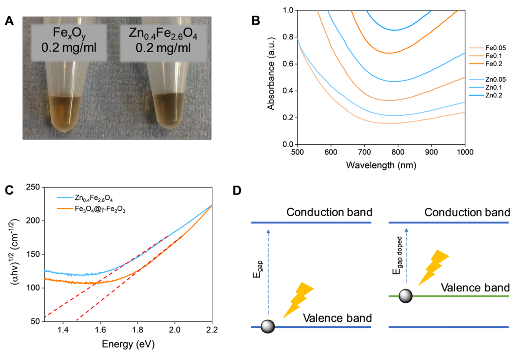
Fig. 5 (A) Digital photographs of \text{Fe}_3\text{O}_4 @ \gamma - \text{Fe}_2\text{O}_3 (left) and \text{Zn}_{0.4}\text{Fe}_{2.6}\text{O}_4 (right) NPs at a concentration of 0.2 \text{ mg}_{\text{Fe+Zn}} \text{ ml}^{-1} . (B) UV-Vis-NIR spectra of \text{Fe}_3\text{O}_4 @ \gamma - \text{Fe}_2\text{O}_3 and \text{Zn}_{0.4}\text{Fe}_{2.6}\text{O}_4 NPs for concentrations between 0.05 – 0.2 \text{ mg}_{\text{Fe or Zn}} \text{ ml}^{-1} . (C) Tauc plots of \text{Fe}_3\text{O}_4 @ \gamma - \text{Fe}_2\text{O}_3 and \text{Zn}_{0.4}\text{Fe}_{2.6}\text{O}_4 NPs with extrapolation of the linear region to y = 0 . (D) A scheme of bandgap decrease by doping.
