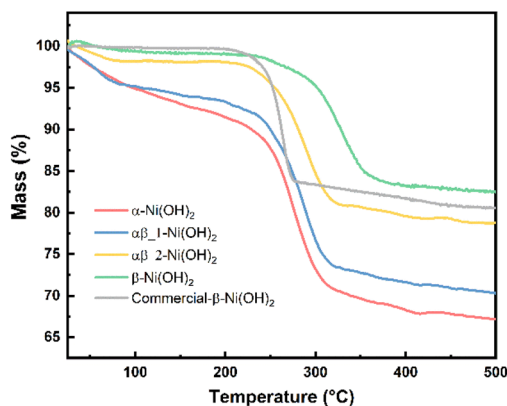
Fig. 5 TGA curves of different phases of nickel hydroxide.
