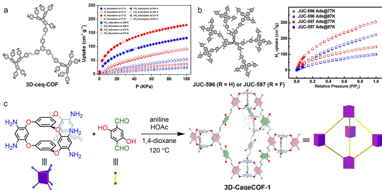
Fig. 5 (a) Schematic representation of 3D-ceq-COF and adsorption–desorption isotherms of \text{H}_2 , \text{CH}_4 , and \text{CO}_2 . Reproduced with permission. 58 Copyright 2020, American Chemical Society. (b) Schematic representation of JUC-596 and JUC-597, and \text{H}_2 adsorption isotherms. Reproduced with permission. 85 Copyright 2022, Wiley-VCH GmbH. (c) Synthesis scheme of 3D-CageCOF-1. Reproduced with permission. 35 Copyright 2020, American Chemical Society.
