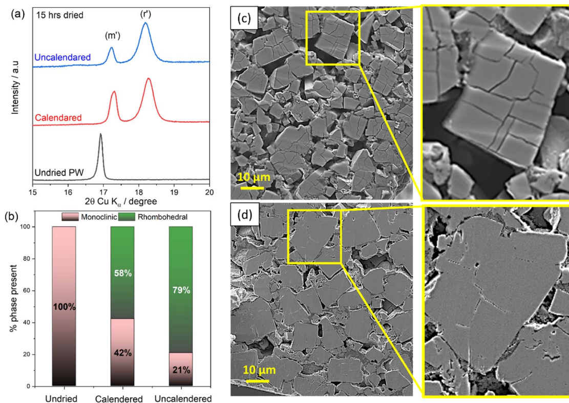
Fig. 6 (a) XRD patterns of calendared and uncalendared electrodes dried for 15 h (170 °C, 10 -3 mbar) relative to a pristine undried PW electrode. (b) Relative percentages of monoclinic and rhombohedral phases calculated for calendared and uncalendared electrodes. Cross-sectional SEM images of (c) uncalendared and (d) calendared pristine electrodes with zoomed areas highlighting internal crack formation.
