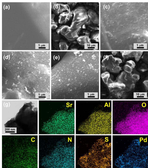
Fig. 3 SEM images of (a and b) AG, (c) AG-MOP-TADS-Pd1, (d and f) AG-MOP-TADS-Pd2, and (e) AG-MOP-TADS-Pd3. (g) EDS-based elemental mapping images of AG-MOP-TADS-Pd2.
