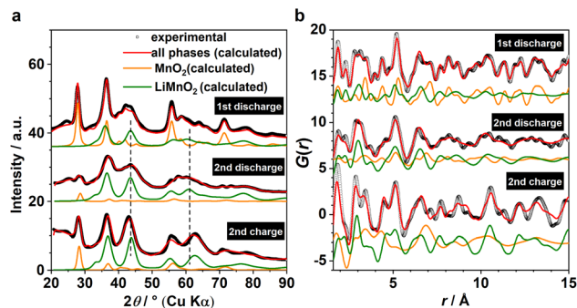
Fig. 4 (a) XRD and (b) PDF joint refinements of the ex situ data for cycled MnO 2 collected at the end of 1st discharge ( R_w^{\text{XRD}} = 3.6\% , R_w^{\text{PDF}} = 32\% ), the end of 2nd discharge ( R_w^{\text{XRD}} = 4.4\% , R_w^{\text{PDF}} = 40\% ) and the end of 2nd charge ( R_w^{\text{XRD}} = 5.0\% , R_w^{\text{PDF}} = 46\% ). Calculated patterns from MnO 2 ( P4_2/mnm , orange) and DRX-LiMnO 2 ( C2/m , green) are shown for comparison. The interfacial intermediate Li 0.5 MnO 2 ( Cmmm ) was omitted for a clearer view. Dashed lines indicate the shift of the Bragg peaks of the DRX phase.
