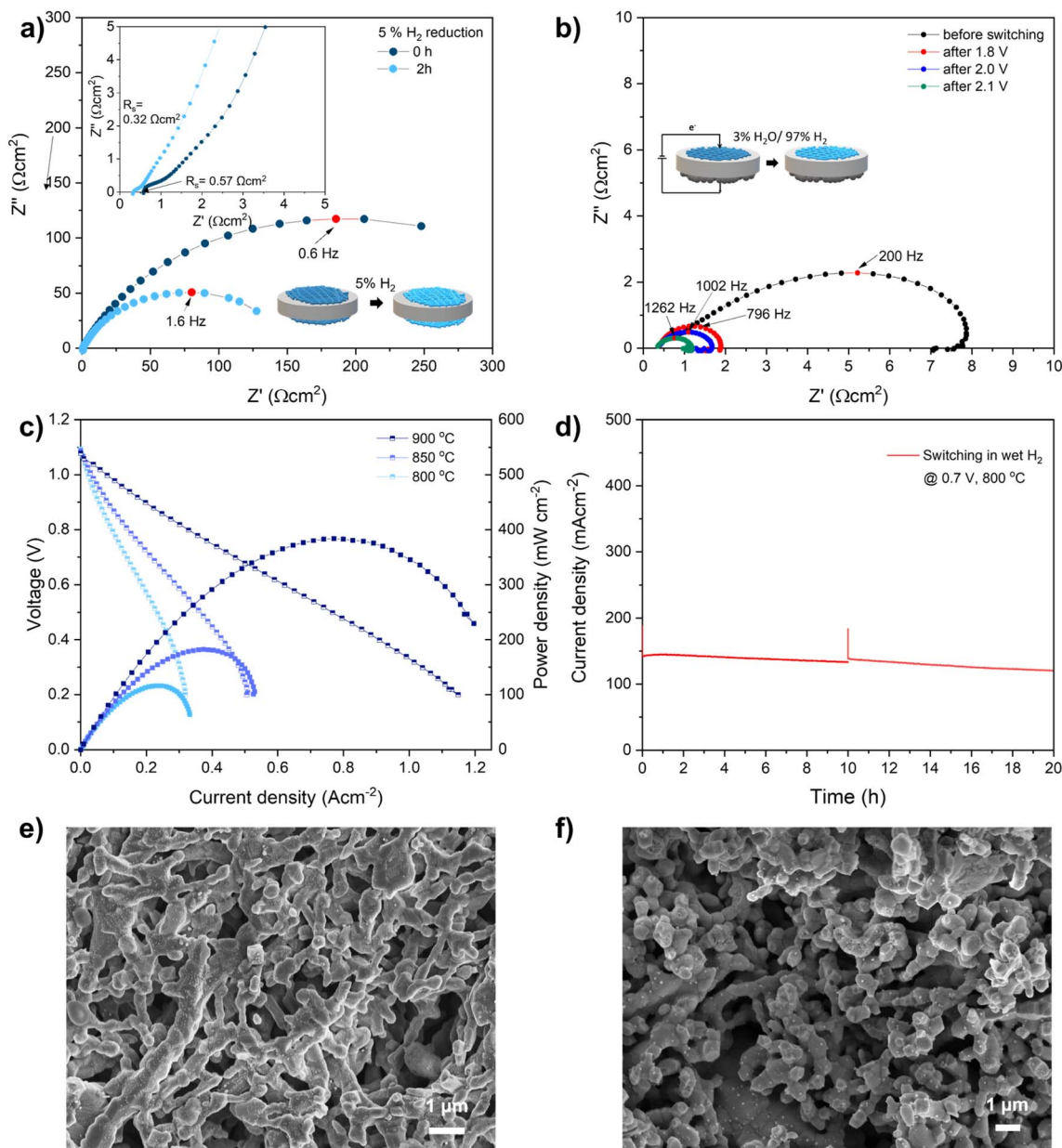
Fig. 5 Performance and short-term stability of fiber electrode-based fuel cells. (a) Impedance spectra of the symmetric cells reduced at 800 °C in 5% H_2/N_2 for 0 and 2 h. (b) Impedance spectra after switching for 180 s at 900 °C at OCV in ~3% H_2O/97\% H_2 . (c) current–voltage–power curves of the cell at different temperatures after switching in wet H_2 . (d) Short term stability in wet H_2 for 20 h. SEM figure of (e) fiber electrode surface in symmetric cell after reduction, (f) fiber electrode in cell after stability test.
