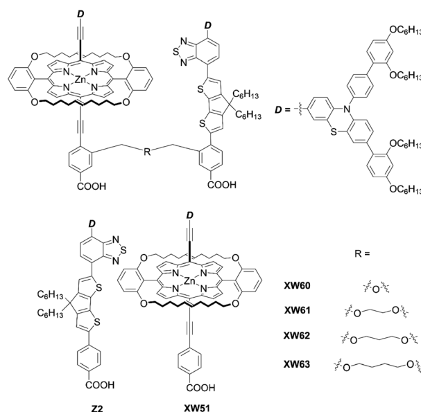
Fig. 18 Chemical structures of XW60–63 , XW51 , and Z2 .
