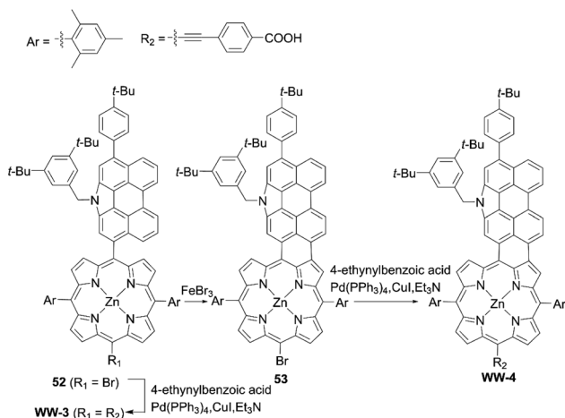
Scheme 11 Synthesis of WW-4 .
