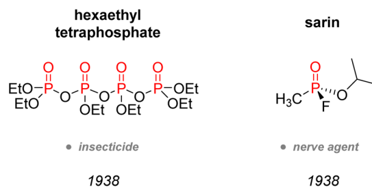
Fig. 2 Timeline of the discovery of significant phosphorus-containing compounds.
