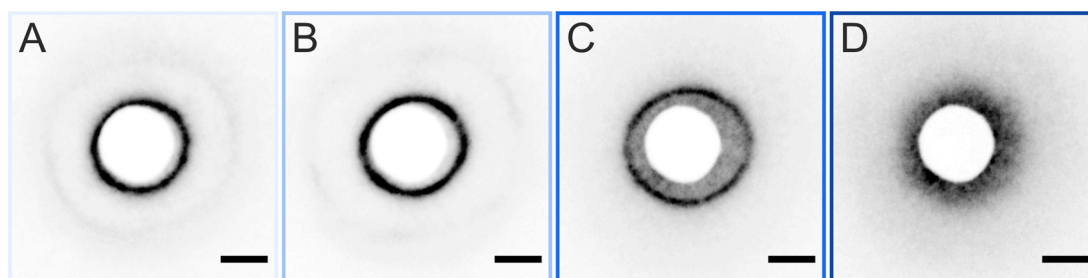
Fig. 2 Scattering patterns of the dried CS microgel monolayer. The corresponding surface pressures ( \Pi ) are (A) 0.5 mN m -1 , (B) 6 mN m -1 , (C) 19 mN m -1 , and (D) 24 mN m -1 . The scale bars correspond to 10 mm.
