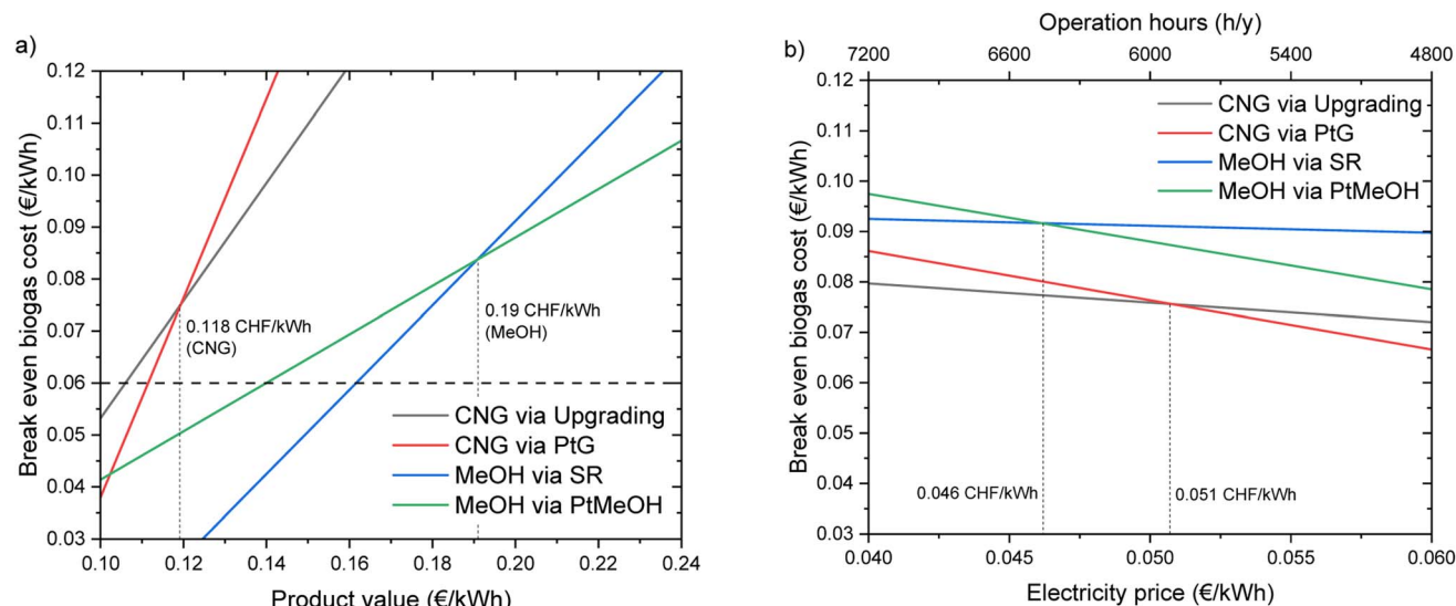
Fig. 9 Sensitivity analysis of the economic assessment for CNG and methanol production: (a) sensitivity to the product price; (b) sensitivity to the electricity price.
