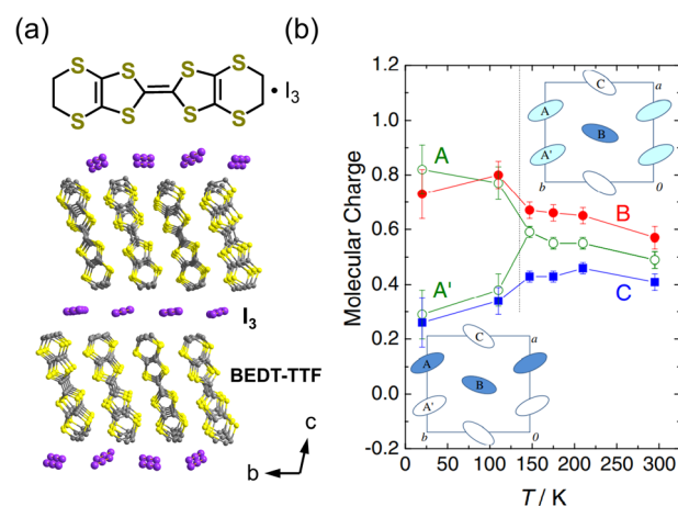
Fig. 7 (a) Crystal structure of \alpha - (\text{BEDT-TTF})_2\text{I}_3 (BEDT-TTF = bis(ethylene)dithio)-tetrathiafulvalene). (b) Temperature dependence of the molecular charge. 43 Reproduced with permission from ref. 43, The Physical Society of Japan.
