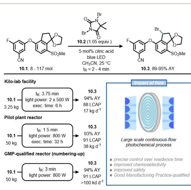
Fig. 10 Adoption of flow chemistry in an industrial setting to improve chemoselectivity and facilitate scalability in the synthesis of 10.3 , an intermediate en route to belzutifan.
