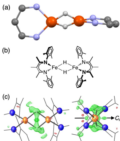
Fig. 1 (a) Ball-and-stick model showing the core of the X-ray crystal structure of 1 at 223 K, 35 emphasizing that the \beta -diketiminate supporting ligands are perpendicular to one another. The pairs of Fe centers and the pairs of hydrides are rendered crystallographically equivalent by the operator -x, y, \frac{3}{2} - z . (b) Chemical structure of 1 , showing the composition of the diketiminato ligands. (c) Two views of the previously reported X-ray crystal structure of 1 at 223 K (left: along the 2-fold axis; right: along the Fe–Fe axis), with the Fe and N atoms as thermal ellipsoids. The residual electron density ( F_{obs} - F_{calc} ) is shown as a green wireframe.
