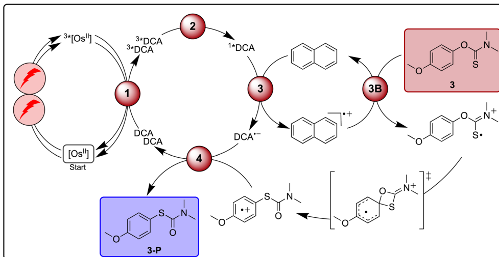
Fig. 5 Light-driven Newman–Kwart rearrangement of substrate 3 under red-light irradiation, along with a plausible mechanism including triplet–triplet energy transfer ( 1 ), triplet–triplet annihilation upconversion ( 2 ), excited state quenching by naphthalene mediator ( 3 ), substrate activation ( 3B ), and catalyst recovery ( 4 ). The main steps of substrate activation are analogous those postulated previously for a monophotonic mechanism. 122,123 A possible radical chain propagation pathway and previously proposed off-cycle intermediates are omitted for simplicity. 122–124 Yield (conversion in parenthesis) was determined by ^1\text{H-NMR} spectroscopy against 1,4-dioxane as internal standard. Further information is in Section 4.6 of the ESI.†
