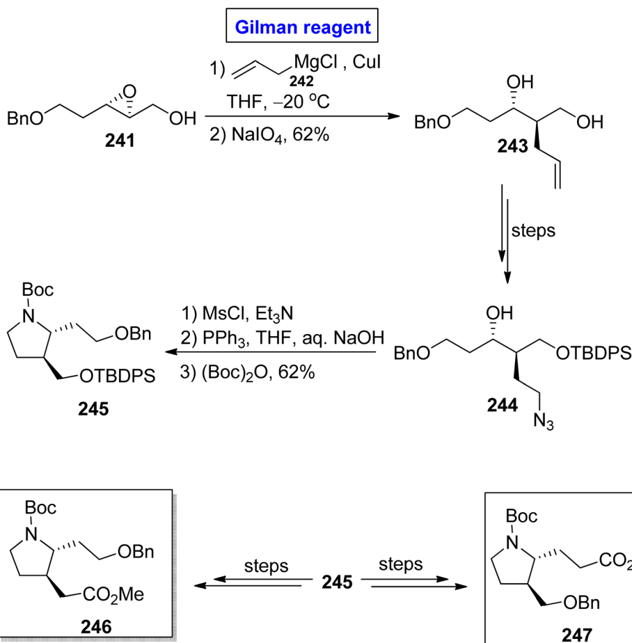
Scheme 28 Synthesis of substituted \beta^{2,3} -proline \text{246} and \beta^3 -homoproline \text{247} .
