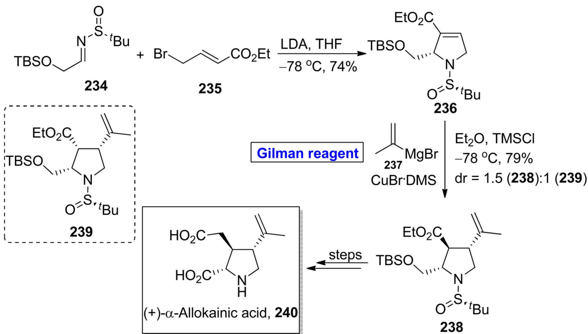
Scheme 27 Synthetic approach towards (+)- \alpha -alkokainic acid \text{240} .
