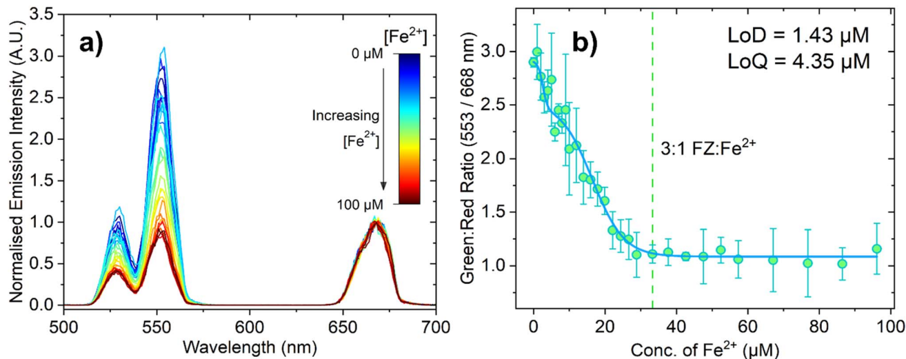
Fig. 5 (a) Emission spectrum of ferrozine (100 \mu\text{M} ) in pH 5.6 MES buffer (0.1 M) with 150 \mu\text{L} \text{NaYF}_4:\text{Yb}^{3+},\text{Er}^{3+} -doped UCNPs with increasing concentration of \text{Fe}^{2+} ions. The spectra have been normalised to the peak centred at 668 nm. This spectrum shows an example of one repeat, where three repeats were conducted overall. The emission monochromator bandwidth was set to 13 nm. (b) The ratio between the intensity of the green (554 nm) and red (668 nm) peaks at each concentration of \text{Fe}^{2+} , with the error bars representing standard deviation over three repeats. The green dashed line represents the concentration at which the 3 : 1 FZ: \text{Fe}^{2+} complex is expected to form (33.33 \mu\text{M} \text{Fe}^{2+} ). Data fitted using a biphasic dose response function in OriginPro®.
