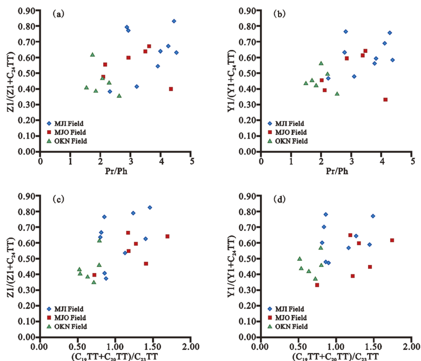
Fig. 11 Cross plots of (a) Z1/(Z1 + C_{24}TT) vs. Pr/Ph, (b) Y1/(Y1 + C_{24}TT) vs. Pr/Ph, (c) Z1/(Z1 + C_{24}TT) vs. (C_{19} + C_{20})TT/C_{23}TT , and (d) Y1/(Y1 + C_{24}TT) vs. (C_{19} + C_{20})TT/C_{23}TT in source rock extracts from Offshore Niger Delta Basin, Nigeria. 169,170
