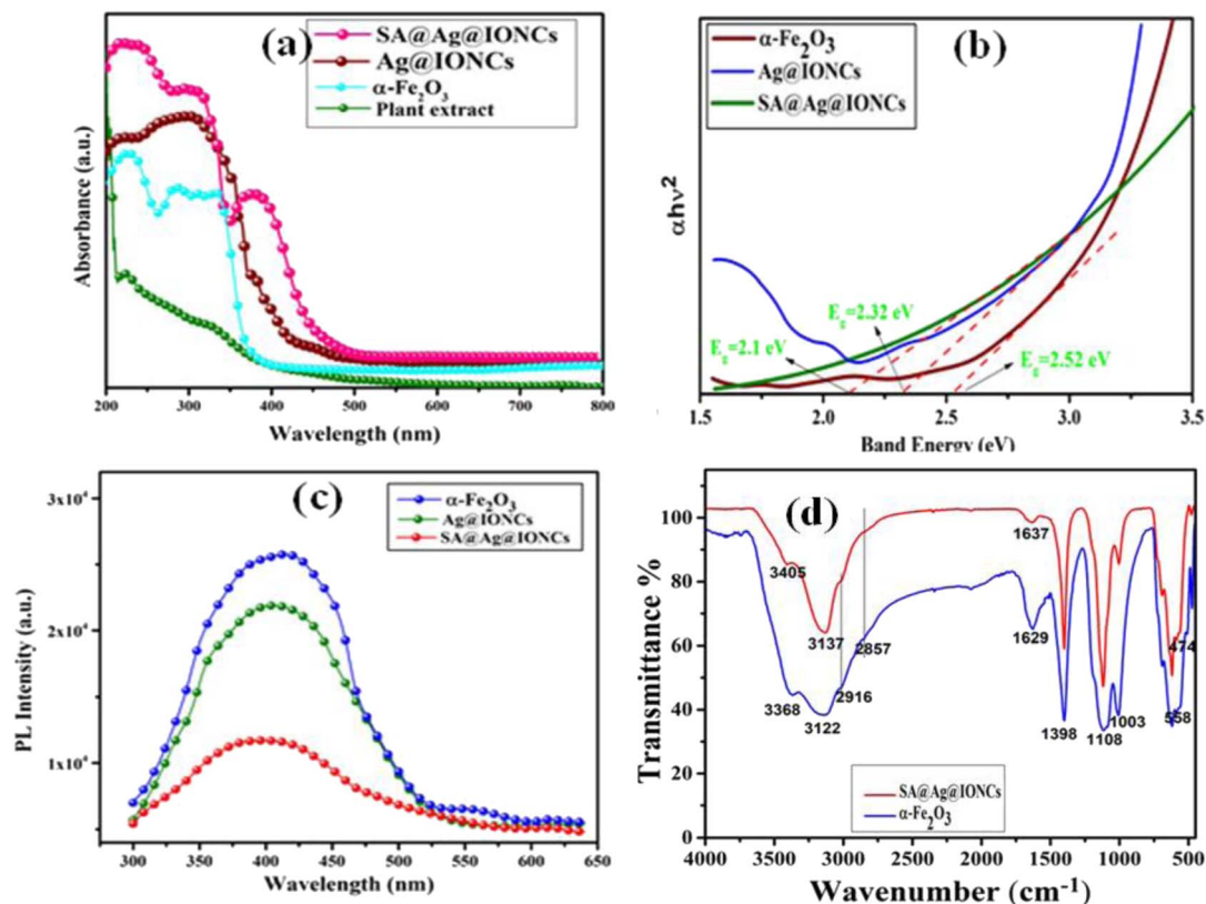
Fig. 7 UV-visible spectra of plant extract, α-Fe 2 O 3 and SA@Ag@IONCs (a), Tauc plot (b), PL spectra (c), and FTIR spectra (d).
