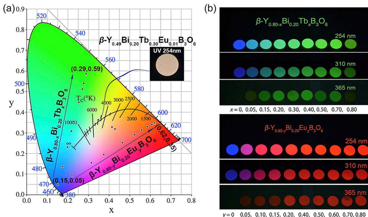
Fig. 1 (a) 1931 Commission Internationale de l'éclairage (CIE) diagram and corresponding positions of Eu 3+ and Tb 3+ -doped phosphors as a function of colour temperature and purity. The inset shows a white light phosphor under UV excitation at 254 nm. (b) The range of emission colours achieved by doping β-YBiB 3 O 6 with different amounts of Tb 3+ (top) and Eu 3+ (bottom) under 254, 310 and 365 nm UV wavelengths. Reproduced with permission from ref. 29.
