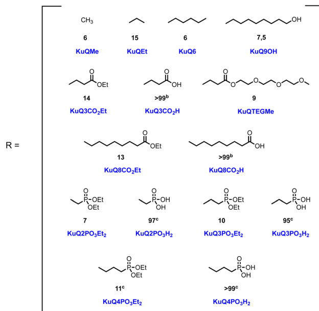
Scheme 1 One-pot synthesis of KuQ derivatives. Reaction conditions: 2-hydroxy-1,4-naphthoquinone 5.75 mmol, alkyl bromide 12 mmol, Cs_2CO_3 8 mmol, ferrocene (Fch) 0.033 mmol, DMSO 22 mL, 41 h, 114 °C. 23,25–27 (a) isolated yield; (b) quantitatively obtained through hydrolysis of the corresponding ester. Reaction conditions: 25 KuQXCO 2 Et (X = 3 or 8) 0.1 mmol in 8 mL THF, NaOH 25% in 2 mL MeOH, 1 h, rt. (c) Quantitatively obtained through hydrolysis of the corresponding phosphonate ester. Reaction conditions: 26 KuQXPO 3 -Et 2 (X = 2, 3 or 4) 0.1 mmol, NaI 5 mmol, bromotrimethylsilane 5 mmol, 16 mL dry CH_3CN:CHCl_3 , 4 h, 40 °C, N_2 atmosphere. Then 30 mL MeOH, 1 h, rt.
