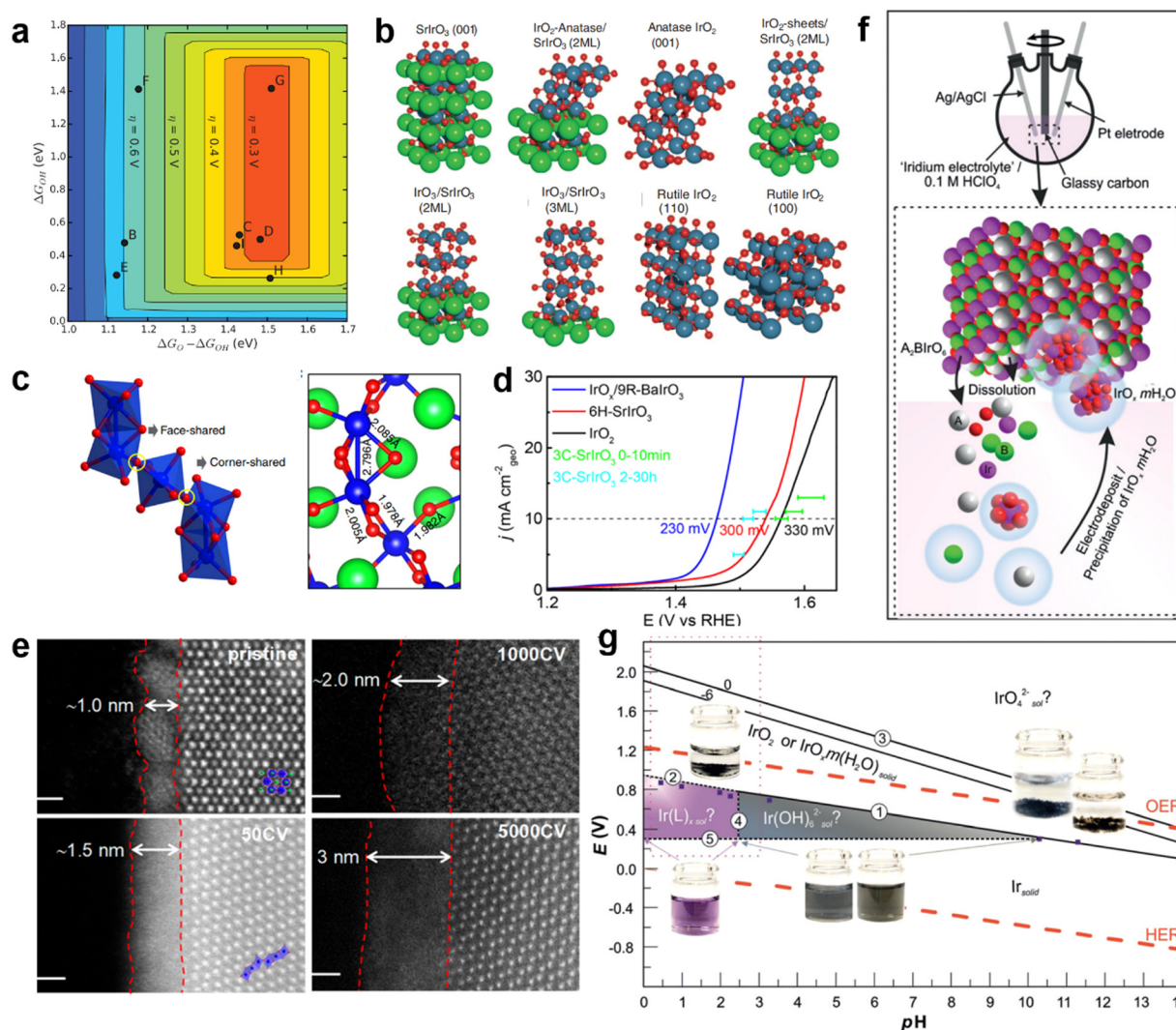
Fig. 10 (a) The theoretical overpotential of IrO_x with different structures exists on the surface with O^* and OH^* binding energies as the descriptor. (b) The model of the surface of IrO_x with different structures. Reproduced with permission. 116 Copyright 2016, American Association for the Advancement of Science. (c) Crystal structure of 6H-SrIrO 3 and different connection modes of IrO_6 octahedron. Reproduced with permission. 117 Copyright 2018, Springer Nature. (d) LSV curves of IrO_x /9R-BaIrO 3 , IrO_2 , and 6H-SrIrO 3 in 0.5 M H 2 SO 4 . (e) HAADF-STEM image of the IrO_x /9R-BaIrO 3 surface after a CV test with different times. Reproduced with permission. 118 Copyright 2021, American Chemical Society. (f) The proposed OER catalytic mechanism in Ir-based perovskite oxidation species involves iridium dissolution-electrodeposition. (g) Iridium E_h -pH diagram. Reproduced with permission. 119 Copyright 2019, Wiley-VCH.
