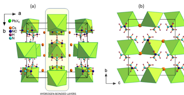
Fig. 1 The crystal structures of \text{Cs}_2\text{MHy}_2\text{PbX}_6 and \text{MHy}^+ are disordered. (a) Discrete (0D) \text{Pb}(\text{Br/I})_6 units interact through HBs with \text{MHy}^+ cations forming HB layers perpendicular to the a direction, coulombic interactions between caesium ions and \text{Pb}(\text{Br/I})_6 units stabilize the structure perpendicular to the layers. (b) The view along the a direction.
