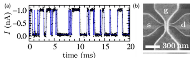
Fig. 23 (a) RTN for a silicon NW on a silicon-on-insulator (SOI) wafer with length of 200 nm and width of 30 nm with SiO 2 gate oxide thickness of 24 nm. V_{GS} = 0.5 V, V_{DS} = -6 mV. (b) Top view of NW. Adapted from ref. 59 with permission. Copyright 2006 Springer.
