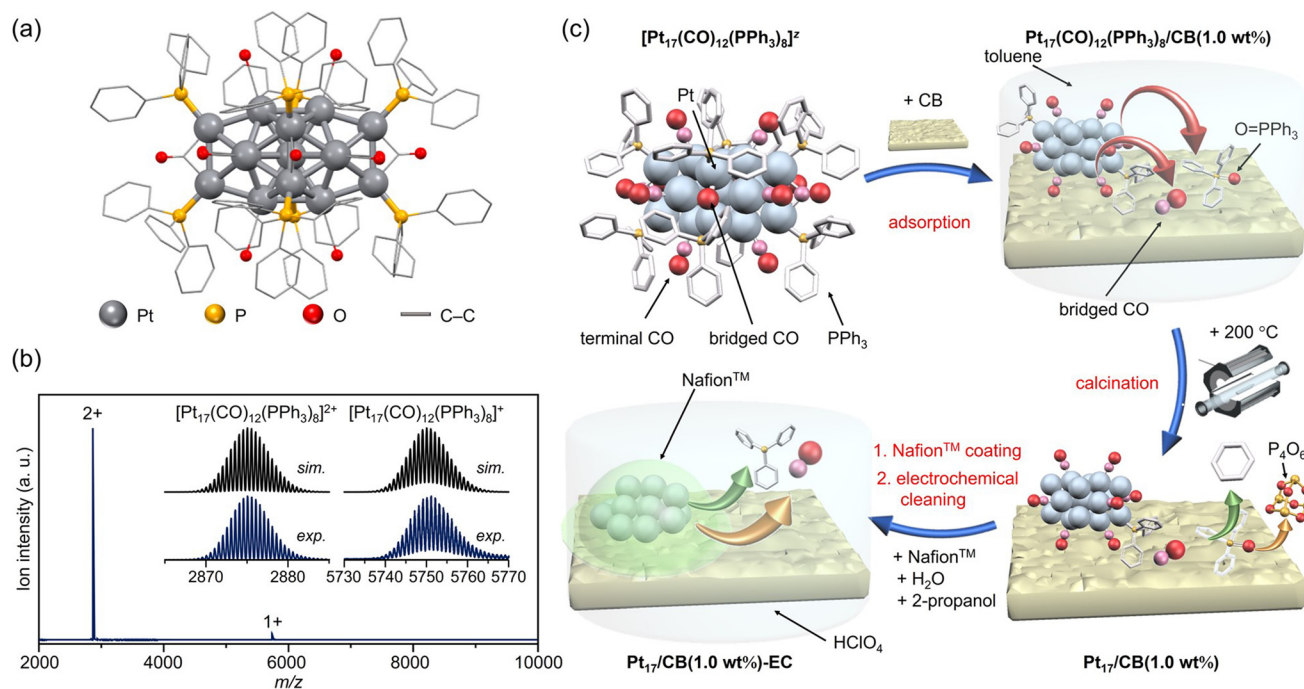
Fig. 1 Preparation of Pt 17 /CB. (a) Geometric structure and (b) ESI-MS spectrum of precursor [\text{Pt}_{17}(\text{CO})_{12}(\text{PPh}_3)_8]^z . (c) Schematic of the preparation procedure: adsorption of [\text{Pt}_{17}(\text{CO})_{12}(\text{PPh}_3)_8]^z onto CB, calcination of the catalyst at 200 °C, and slurry preparation. In (c), the states of the ligand at each stage are estimated based on the results of the FT-IR spectroscopy (Fig. 3 and S10†), HAX-PES (Fig. S11†), FT-EXAFS (Fig. 4(a)), XANES (Fig. 4(b)), and TGA (Fig. S18†) analyses.
