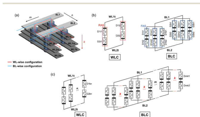
Fig. 4 The vertical 2 \times 2 crossbar array structure. (a) The three-layered structure and its configurations. The equivalent circuit of configurations when (b) n = 2 , m = 2 , and (c) for a larger size. The high parallel FAS gates indicated in blue dotted boxes can be achieved in the BLC. The number of possible circuits in the BLC is dependent on k .
