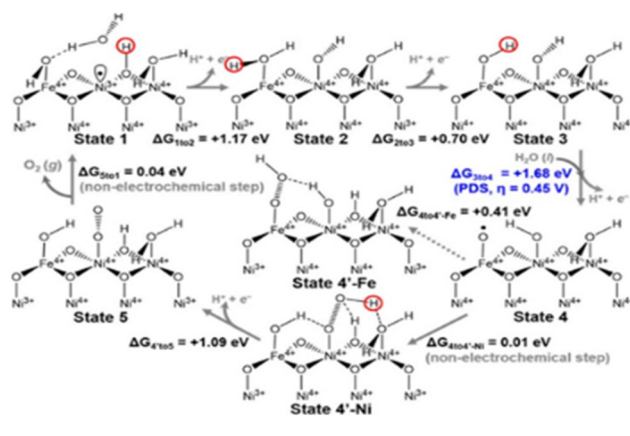
Fig. 3 Mechanism of the OER on the Ni 1-x Fe x OOH catalyst leading to \eta = 0.45 V. Reproduced with permission from ref. 73: Copyright 2018, American Chemical Society.
