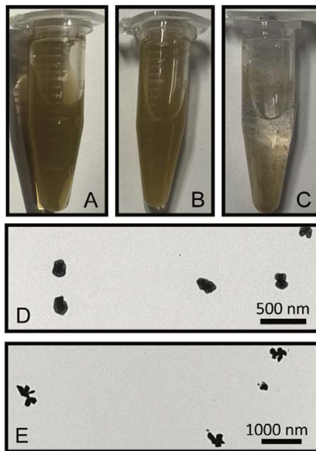
Fig. 7 Photographs of the nanotags (A), nanosupernova (B) and the \text{Au}/\text{AgNSs}@\text{Ag} particles (C). The nanotags and nanosupernova are stable in solution, however when no DTNB is added the particles aggregate. TEM images of particles made using the synthesis method for nanotags (D) and nanosupernova (E), but without the addition of hydroquinone.
