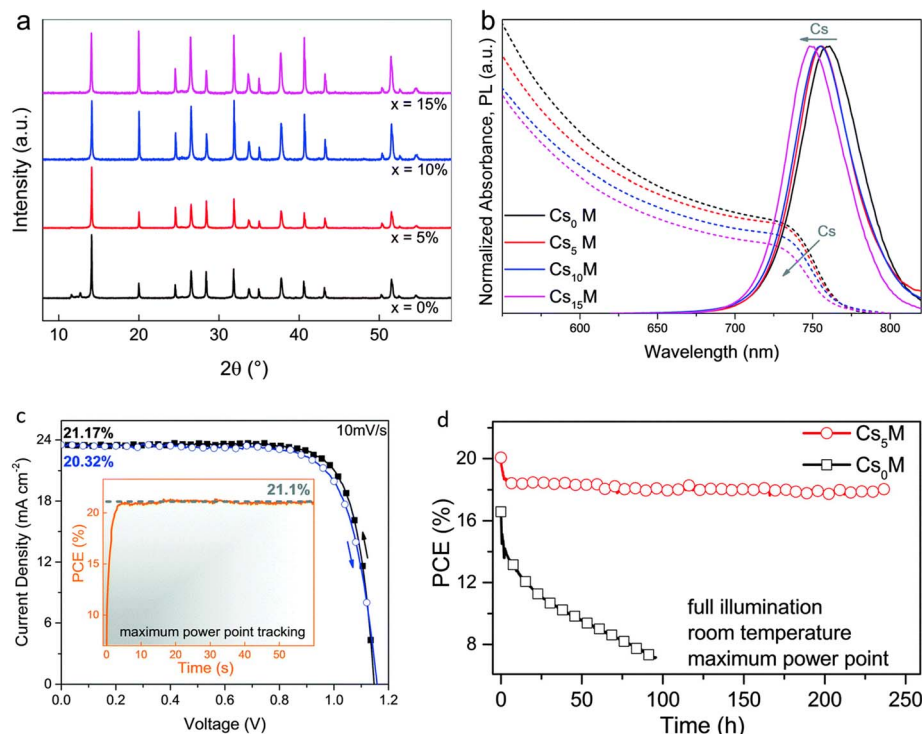
Fig. 8 Consequences of Cs accumulation in MA/FA cation blends; (a) XRD and (b) optical findings (c) current–voltage ( J-V ) and (d) stability properties of \text{Cs}_x\text{MAFA} complexes (reproduced with permission from ref. 60. Copyright 2017 RSC).
