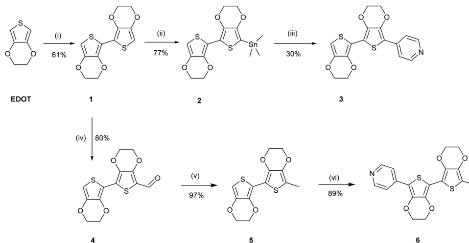
Scheme 2 Reagents and conditions: (i) THF, n -BuLi, -80^{\circ}\text{C} , then \text{CuCl}_2 , 0^{\circ}\text{C} , 16 h. (ii) THF, n -BuLi, -80^{\circ}\text{C} , then \text{SnMe}_3\text{Cl} , rt, 16 h. (iii) THF, \text{Pd}(\text{PPh}_3)_4 , 4-bromopyridine, reflux, 48 h. (iv) Dichloroethane (DCE), DMF, \text{POCl}_3 , 0^{\circ}\text{C} , then 80^{\circ}\text{C} , 18 h. (v) Ethylene glycol, \text{NH}_2\text{NH}_2 , KOH, 130^{\circ}\text{C} , 1 h, then 180^{\circ}\text{C} , 16 h. (vi) DMF, 4-iodopyridine, KOAc, \text{Pd}(\text{OAc})_2 , 80^{\circ}\text{C} , 16 h.
