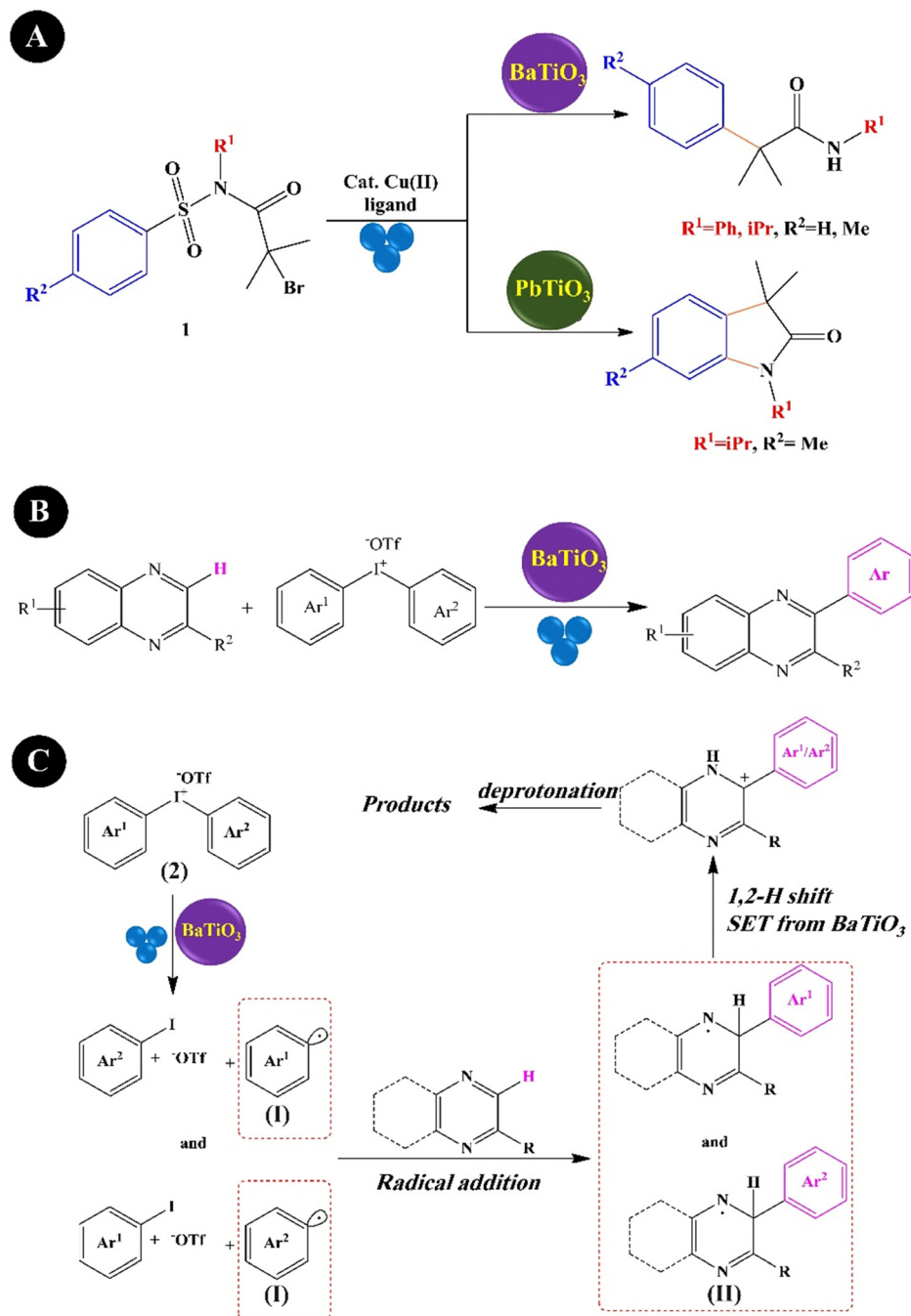
Fig. 12 Mechano-induced synthesis of \alpha -arylamides and oxindoles (A) (adapted from ref. 214 with permission from John Wiley and Sons). The procedure (B) and mechanism (C) of mechano-induced C(sp 2 )-H arylation of quinoxalin(on)es (adapted from ref. 215 with permission from Elsevier).
