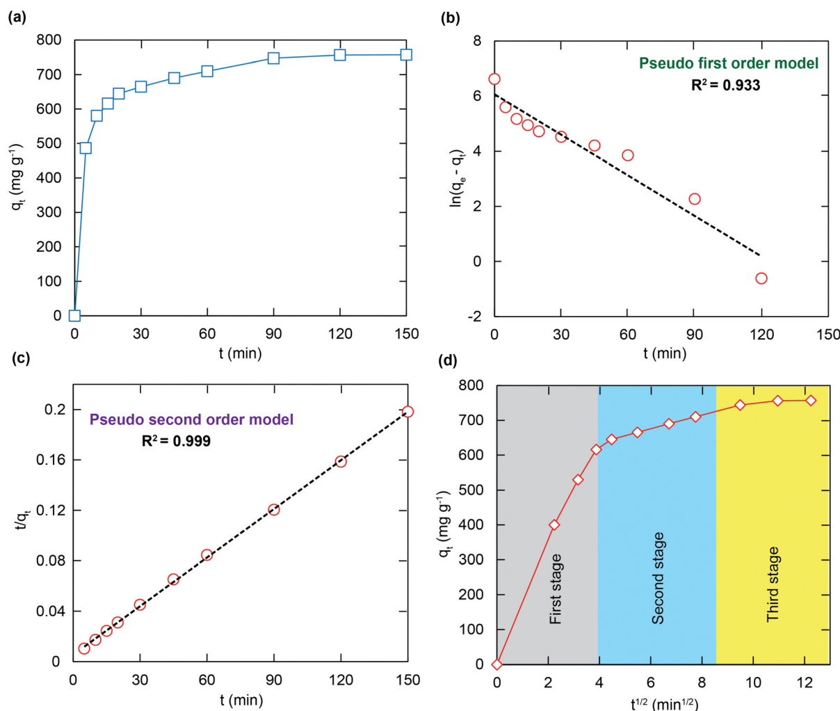
Fig. 6 The kinetic curve for the adsorption of RhB onto \text{H}^+ \text{C} \text{BUT-8}(\text{Cr}) [ m = 10 \text{ mg} , V_{\text{RhB}} = 100 \text{ mL} , C_o = 100 \text{ mg L}^{-1} , \text{pH} = 3 ] (a); data fitting with the adsorption kinetic models: pseudo first order (b), pseudo second order (c) and intra-particle diffusion model (d).
