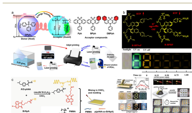
Fig. 4 (a) Energy transfer between donor (host) and acceptor (guest) and molecular structures of acceptors; the production of anti-counterfeiting marks using inkjet printing (reproduced with permission from ref. 54. Copyright 2021, Wiley-VCH GmbH). (b) Illustration of acid-alkali responsive structure of R/S-BPNAp and R/S-BPHP. Photographs of number “8” written using aqueous R-BPHP and “5” written using aqueous R-BPNAp on the same number “8” (reproduced with permission from ref. 55. Copyright 2021, Elsevier B.V.). (c) Schematic illustration of the structure and preparation of the p(phNA-co-BrNpA)-PMMA film and its anti-counterfeiting application (reproduced with permission from ref. 56. Copyright 2022, Springer Nature).
