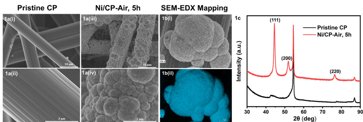
Fig. 1 (a) (i & ii) SEM images of pristine carbon paper (CP); (iii & iv) CP after electroplating from a 40 mM solution of NiCl 2 ·6H 2 O for 5 h under air (Ni/CP-Air); (b) (i & ii) SEM & EDX elemental mapping of Ni/CP-Air; (c) XRD spectrum of pristine CP & Ni/CP-Air.
