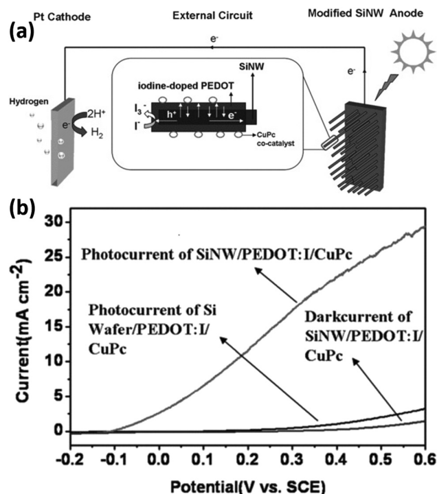
Fig. 25 (a) Schematic diagram of the hydrogen-production PEC cell. (b) PEC performance comparison of the different photoelectrodes. Reproduced with permission from ref. 160, Copyright © 2012 Wiley-VCH Verlag GmbH & Co. KGaA, Weinheim.
