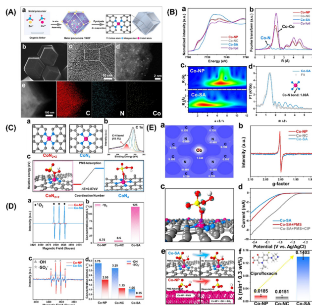
Fig. 7 (A) Preparation steps of Co-SA. (b)–(e) SEM, TEM, HAADF-STEM and EDS mapping images of Co-SA. (B) (a) Co normalized K-edge XANES spectra and (B) K^3 -weighted Fourier transform spectra of Co foils and Co-based samples. (c) Wave transformations of Co-NP and Co-SA. (d) EXAFS fitting curve corresponding to Co-SA in R space. (C) Atomic structure of \text{CoN}_{2+2} and \text{CoN}_4 active sites of Co-SA (a) and XPS spectrum of C of Co-SA (b). The free energy evolution of the active sites for PMS adsorption of \text{CoN}_{2+2} and \text{CoN}_4 (c). (D) EPR spectrum and quantitative determination of ^1\text{O}_2 , ^{\bullet}\text{OH} and \text{SO}_4^{\bullet-} . (E) Two-dimensional valence electron density map of the \text{CoN}_{2+2} site in Co-SA (a). EPR spectrum of catalysts (b). The electron density difference diagram (c) of Co-SA and PMS adsorbed at the \text{CoN}_{2+2} site. (d) Linear sweep voltammetry (LSV) curves of Co-SA. (e) Adsorption of PMS on Co-SA and Co-NP surfaces. (f) Degradation efficiency of CIP in different systems. Copied with permission from Ref. 21. Copyright 2021, Wiley.
