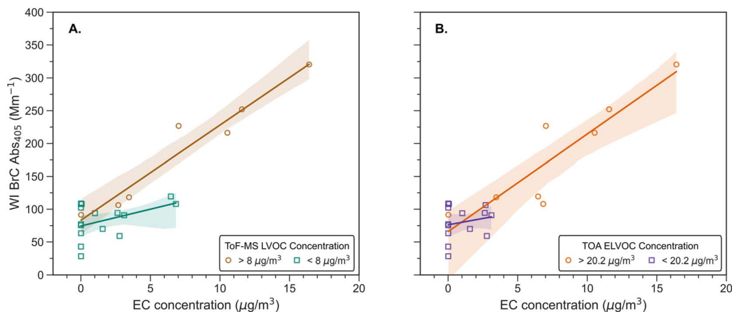
Fig. 3 Dependence of the water-insoluble (WI) BrC light absorption coefficient at 405 nm ( \text{Abs}_{405} ) on EC concentration. The different panels represent regression fits estimated based on the Johnson–Neyman analysis using (A) the ToF-MS based LVOC concentrations and (B) the TOA based ELVOC concentrations as the moderating variables. The circles represent data points for which a change in EC had a significant impact on WI BrC \text{Abs}_{405} and squares represent data where change in EC had minimal effect on WI BrC \text{Abs}_{405} . The solid lines are linear fit lines, and the shaded regions represent 95% confidence intervals.
