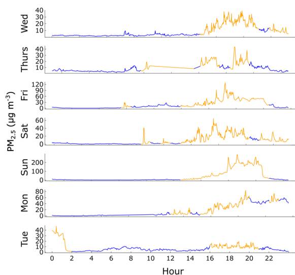
Fig. 8 \sigma_{\Delta\text{PM}} filter applied to unit ccc9 for the first week in December 2021. Blue data points correspond to periods of low \sigma_{\Delta\text{PM}} , yellow data points correspond to periods of high \sigma_{\Delta\text{PM}} .
