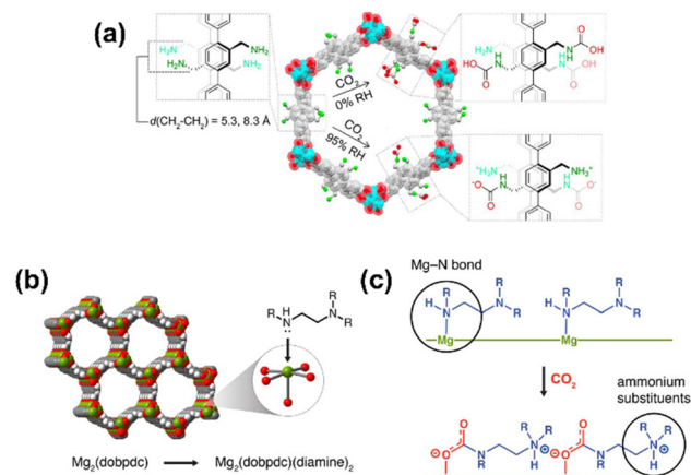
Fig. 5 (a) Chemisorption species post- \text{CO}_2 adsorption in IRMOF-74-III-( \text{CH}_2\text{NH}_2 ) 2 . 35 (b) Representative structure of the metal-organic framework \text{Mg}_2(\text{dobpdc}) . Green, red, gray, and white spheres represent Mg, O, C, and H atoms, respectively. (c) Depiction of cooperative \text{CO}_2 insertion into a row of \text{Mg}^{2+} -diamine sites to form ammonium carbamate chains along the pore axis. 88 Reproduced with permission, Copyright 2017 American Chemical Society.
