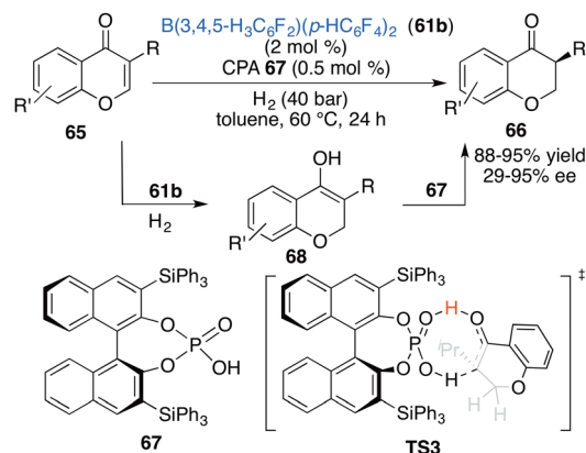
Scheme 33 Asymmetric relay hydrogenation of chromones.
