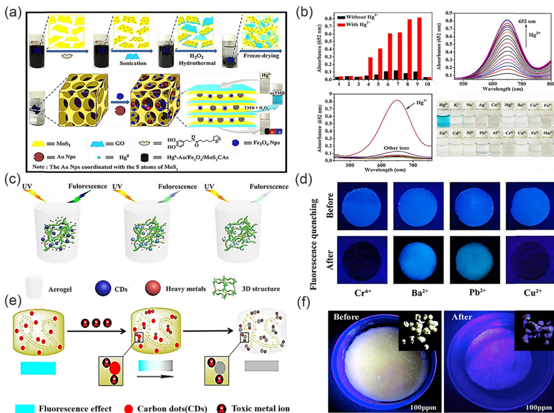
Fig. 16 Synthesis of functional fluorescent aerogels and their mechanism of sensing and removing heavy metal ions. (a) The detection mechanism of Au/Fe 3 O 4 /MoS 2 CAs for Hg 2+ . (b) The fluorescence spectra and adsorption properties of Au/Fe 3 O 4 /MoS 2 C for Hg 2+ . Reproduced from ref. 124 with permission from American Chemical Society. Copyright 2016. (c) The mechanism of the adsorption and fluorescence sensing of Cr(VI). (d) The fluorescence quenching image in presence of different heavy metal ions. Reproduced from ref. 125 with permission from Royal Society of Chemistry. Copyright 2020. (e) The mechanism of detection and removal of heavy metal ions by CQDs/NFC composite aerogel. (f) The optical image of fluorescent aerogel under ultraviolet light before and after adsorption. Reproduced from ref. 126 with permission from Elsevier B.V. Copyright 2020.
