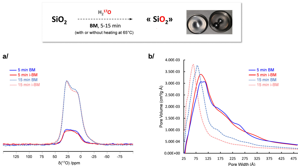
Fig. 4 Influence of i-BM on the isotopic labeling of fumed silica. (a) 17 O MAS NMR spectra, and (b) comparison of the pore size distribution (as determined from N 2 adsorption measurements, using the Barrett, Joyner et Halenda – BJH – model, as in our previous study on the 17 O-labeling of silica), 52 for phases prepared after 5 and 15 minutes milling, with (red) or without (blue) i-BM.
