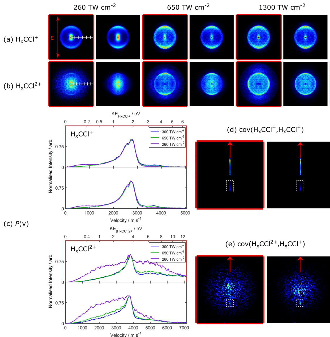
Fig. 6 Symmetrised images of the (a) H_x CCl^+ and (b) H_x CCl_2^{2+} fragments observed following 805 nm SFI of cis - (red borders) and trans -1,2-DCE at I = 260, 650 and 1300\ TW\ cm^{-2} . The laser polarisation vector, \epsilon , is vertical in the plane of the image, as shown in the top left-hand panel and the relative signal intensities are shown by the linear false-colour scale chosen to span the maximum to minimum signal levels in the regions of interest within each image at the end of row (b). The ticks on the white horizontal scale in the left-hand image in each row indicate 1000\ m\ s^{-1} intervals. The P(v) distributions of the H_x CCl^+ and H_x CCl_2^{2+} fragments from each parent isomer are shown in (c) with, in each case, the maximum signal scaled to an intensity of unity. The corresponding fragment kinetic energies are shown on the top x axis. (d and e) Show, respectively, the (H_x CCl^+, H_x CCl^+) and (H_x CCl_2^{2+}, H_x CCl^+) covariance map images from analysis of I = 260\ TW\ cm^{-2} data from the cis - (left) and trans -isomers (right), selecting H_x CCl^+ as the reference ion and fixing its velocity to be vertically upwards, as indicated by the red arrow. The covariance signal of interest in each case is bounded by dashed white lines, while the more intense feature along the \phi = 0^\circ axis in both images in (d) is the autovariance signal.
