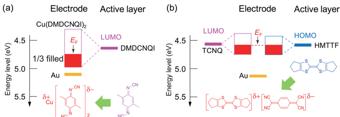
Fig. 5 Energy-level alignment between the semiconductors and electrodes in self-contact (a) DMDCNQI/ \text{Cu}(\text{DMDCNQI})_2 and (b) HMTTF/(HMTTF)(TCNQ) transistors. Reprinted with permission from ref. 88. Copyright 2014, American Chemical Society.
